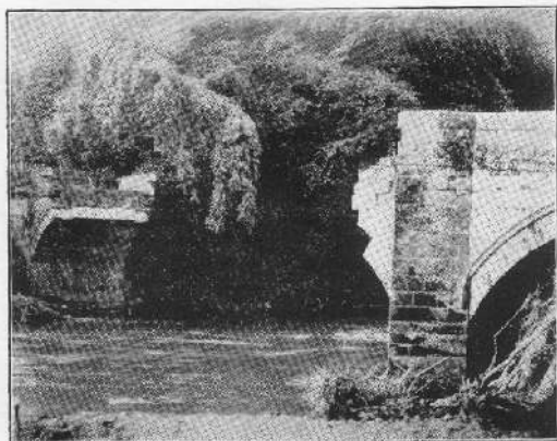
ECTON BRIDGE AFTER FLOOD.
